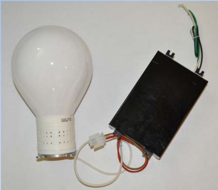
INDUCTION LIGHT
